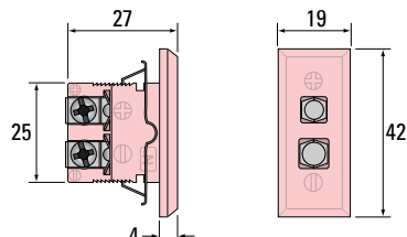
Type N IEC illustrated (R29SN-I). Recommended cutout: 13mm x 26mm
