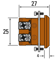
Recommended cutout: 13mm x 26mm. Type K illustrated (R34K)
