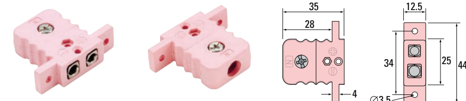
Type N IEC illustrated (R30N-I). Recommended cutout: 13mm x 26mm
