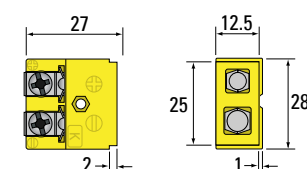
Type K ANSI illustrated (R28K-A) - see page 32 for mounting kit. Recommended cutout: 13mm x 25.8mm
