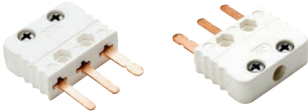
Type CU IEC illustrated (F16CU)
