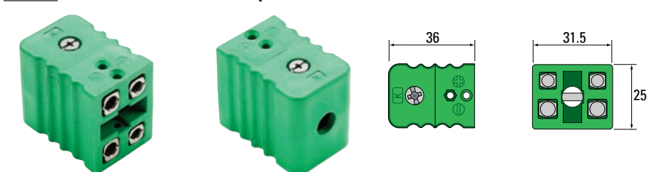
Type K IEC illustrated (R92K-I)
