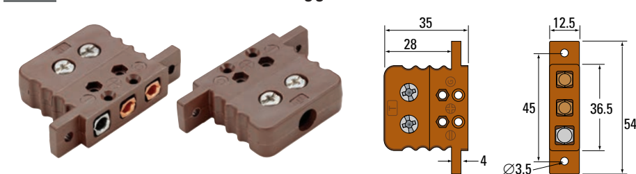
Type T IEC illustrated (R31T-I). Recommended cutout: 13.5mm x 37mm
