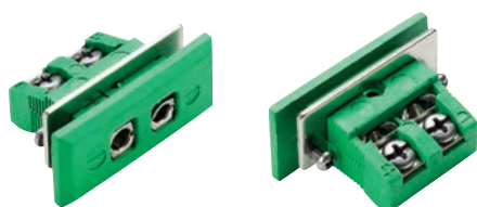
Type K IEC illustrated (R29K-I). Recommended cutout: 13mm x 26mm
