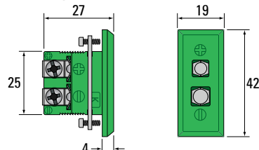
Type K IEC illustrated (R29K-I). Recommended cutout: 13mm x 26mm
