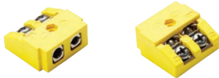
Type K ANSI illustrated (R28K-A) - see page 32 for mounting kit. Recommended cutout: 13mm x 25.8mm
