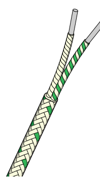
High Temperature Fibreglass Insulated Flat Twin One pair of solid conductors. Cores single HT glass fibre lapped, braided and varnished. Pair laid flat, glass fibre braided and varnished.
