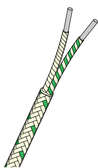
High Temperature Fibreglass Flat Twin One pair of solid conductors. Cores single HT glass fibre lapped, braided and varnished. Pair laid flat, glass fibre braided and varnished.
