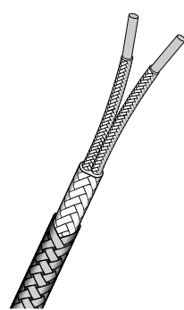
Ceramic Fibre Flat Twin with Inconel 600 Braid One pair of solid conductors. Cores ceramic fibre braided. Pair laid flat, ceramic fibre braided overall. Inconel 600 braid overall.
