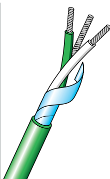
HR PVC Twisted Pair with Screen One pair of stranded conductors. Cores HR PVC insulated. Pair twisted, screened with Mylar aluminium tape and drain wire. HR PVC sheathed overall.
